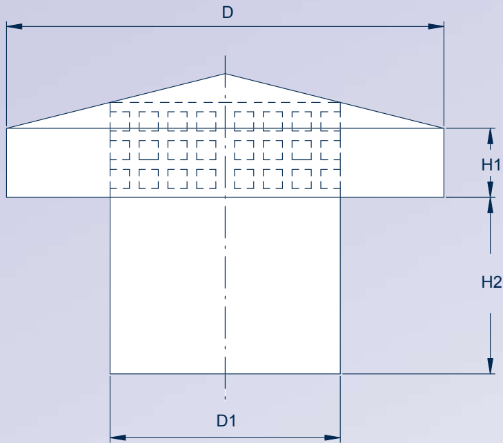
ROOF HOOD – circular –
